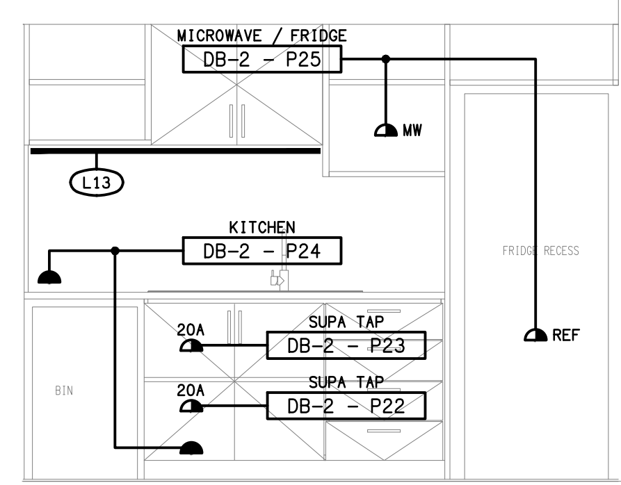
DETAIL A STAFF ROOM KITCHENETTE ELEVATION SCALE 1: 25
